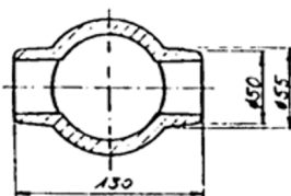
Middle post nr. 2005-4 A, section Y-Y
