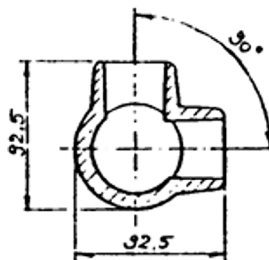
Corner posts nr. 2005-4 B, section Z-Z
