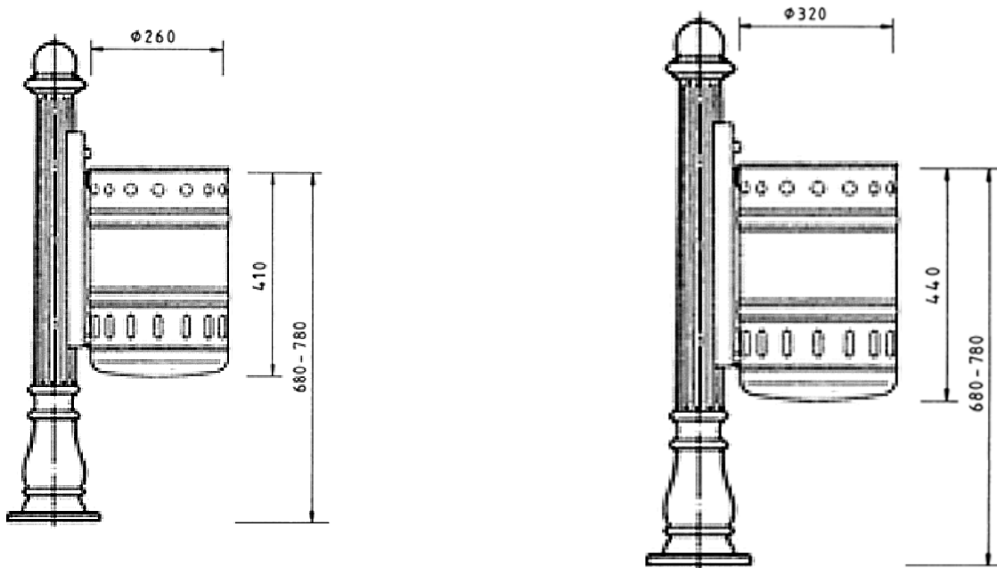
Waste bin TAB-3000.30
